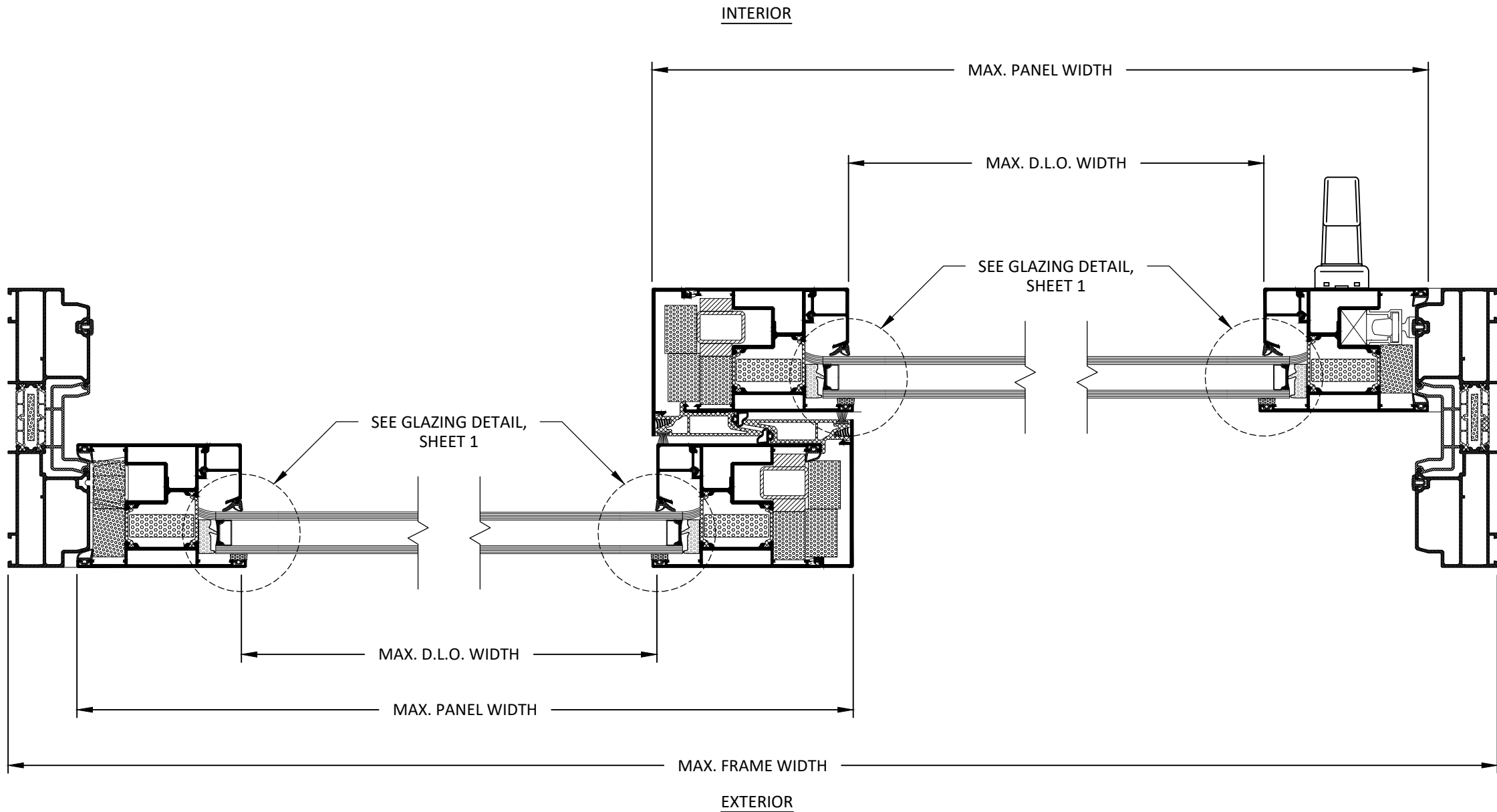
A 4 HORIZONTAL SECTION
