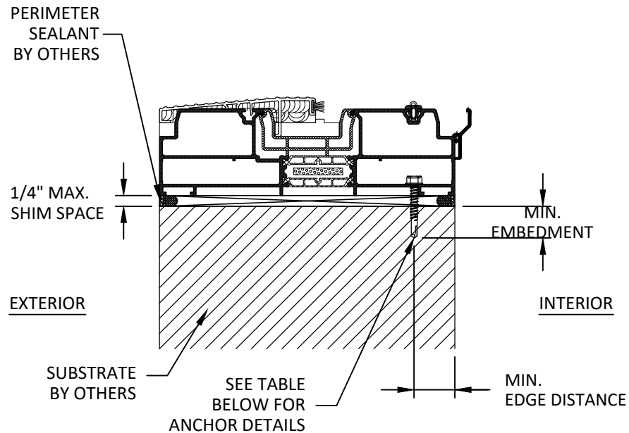
B 5 HORIZONTAL SECTION SILL - THROUGH FRAME
