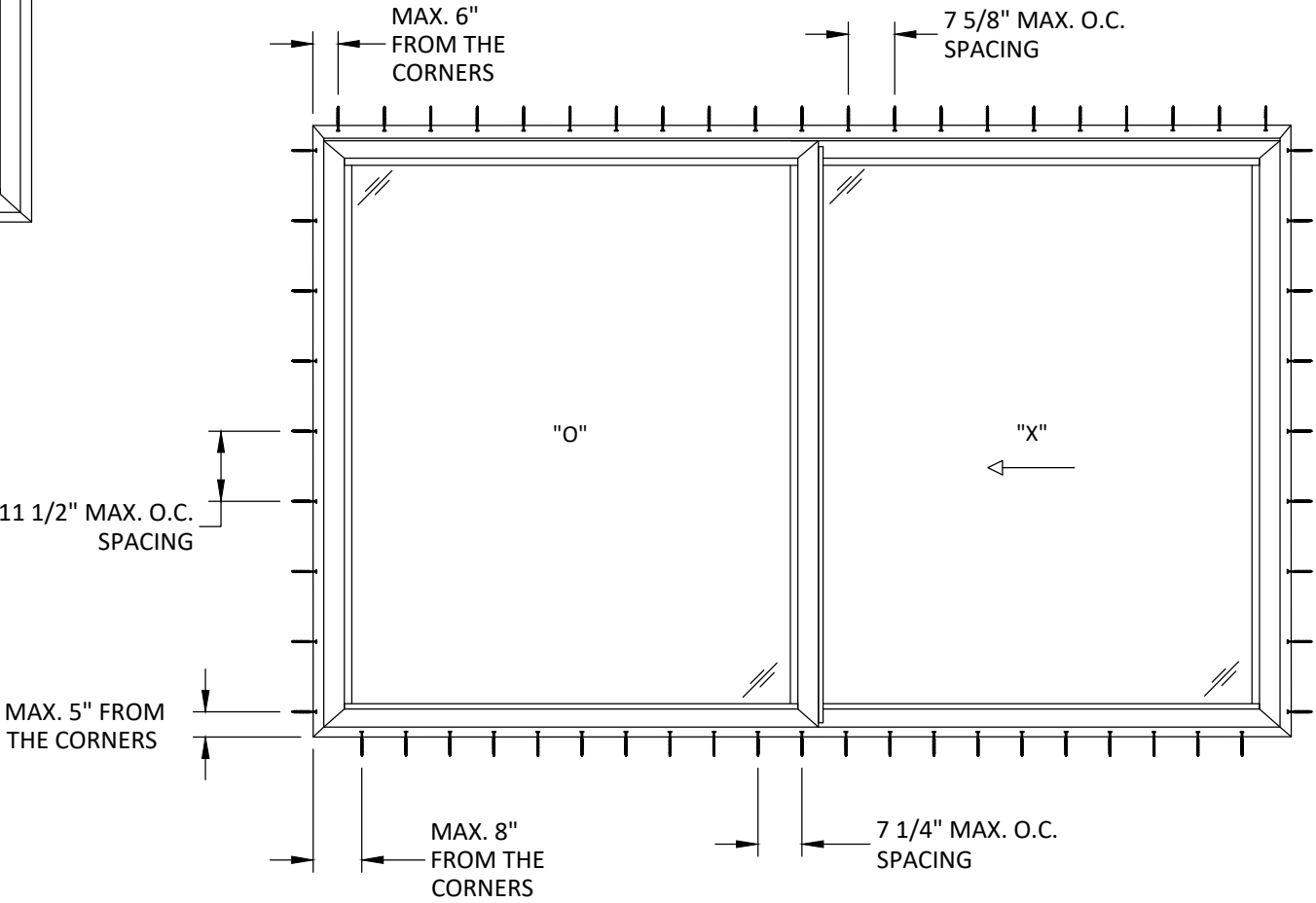
ANCHOR LAYOUT THROUGH FRAME INSTALLATION
