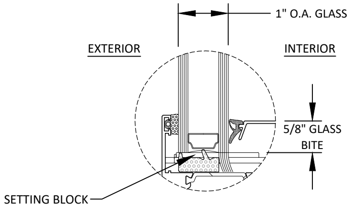
GLAZING DETAIL 1
