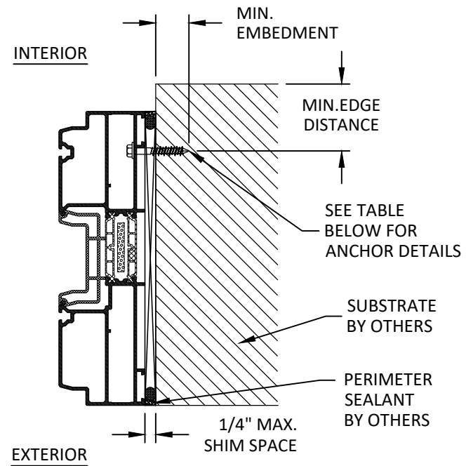
C 5 HORIZONTAL SECTION JAMB - THROUGH FRAME
